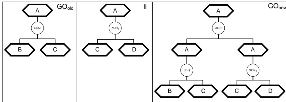
Fig. 10. A generic example of a Global Input diagram ( GO_{old} ), a local input diagram ( li ), and a Global Output diagram ( GO_{new} ). The example illustrates the case in which A^{li} generates a conflict because a counterpart A^{GO} exists that has a different routing type.
