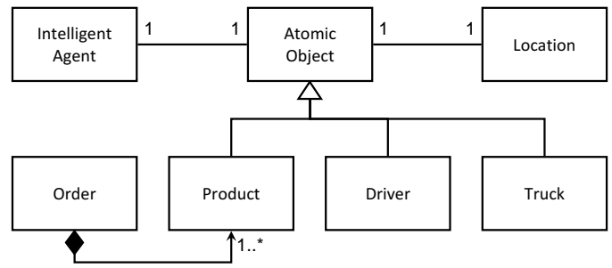
Figure 5: Addition of Product and Intelligent Agent classes in new system design
