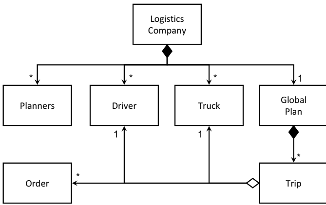
Figure 4: Existing company class diagram
